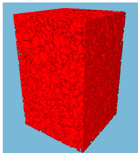
Fig. 2 Dense initial assembly of 6400 ovoid particles, \alpha = 0.50
