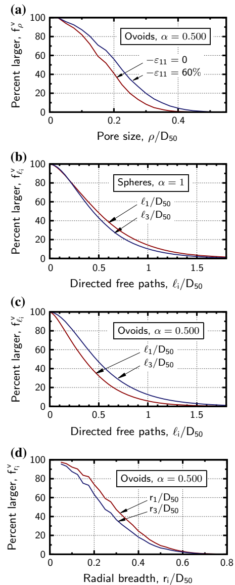
Fig. 11 Distribution of void sizes and orientations: a pore size distribution f_\rho^v for ovoid assemblies ( \alpha = 0.500 ) at strains of 0 and 60% (Eq. 14), b directed free path distributions f_{\ell_i}^v for sphere assemblies in x_1 and x_3 directions at strain 60% (Eq. 15), c directed free path distributions f_{\ell_i}^v for ovoid assemblies ( \alpha = 0.500 ) at strain 60% (Eq. 15), and directed radial breadth distributions f_{r_i}^v for ovoid assemblies ( \alpha = 0.500 ) at strain 60% (Eq. 18)
